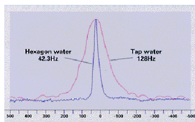
NMR reading of Hexagon water
