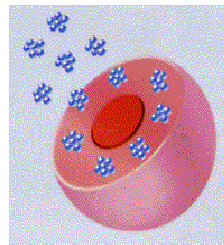
Small water clusters can easily penetrate cells/or improved hydration.
